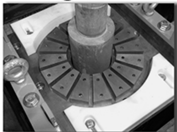
Silver Graphite Anodic Interface For Rotating Internal Anode
